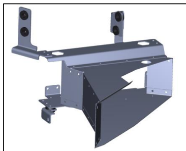
Insulator to reduce the oil pump operation noise.
